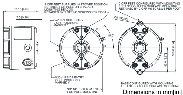
Fig. 1 Fixing Location for Junction Box
