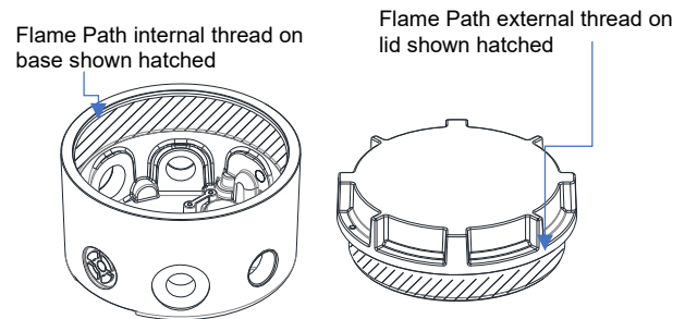
Figure 1: Flame Path.
