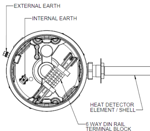
Figure 4: Earth Internal & External
