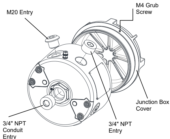
Fig. 2 Accessing the Enclosure.
