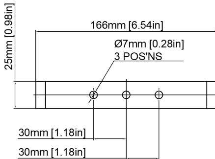
Figure 2: Fixing Location for GNEs2F Sounder.
